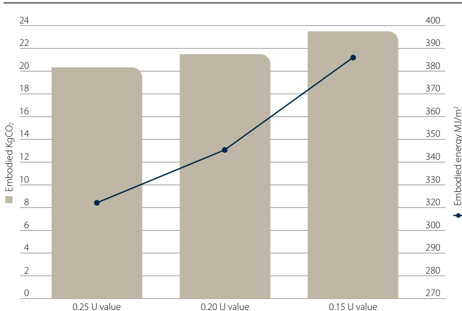
Figure 3. Embodied CO 2 and energy for reducing U values.
