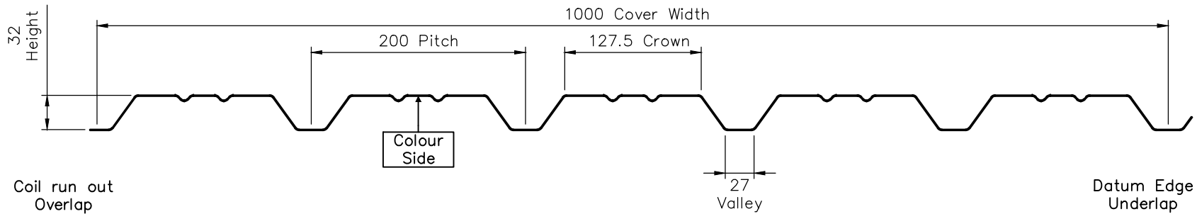
SECTION THROUGH PROFILE
