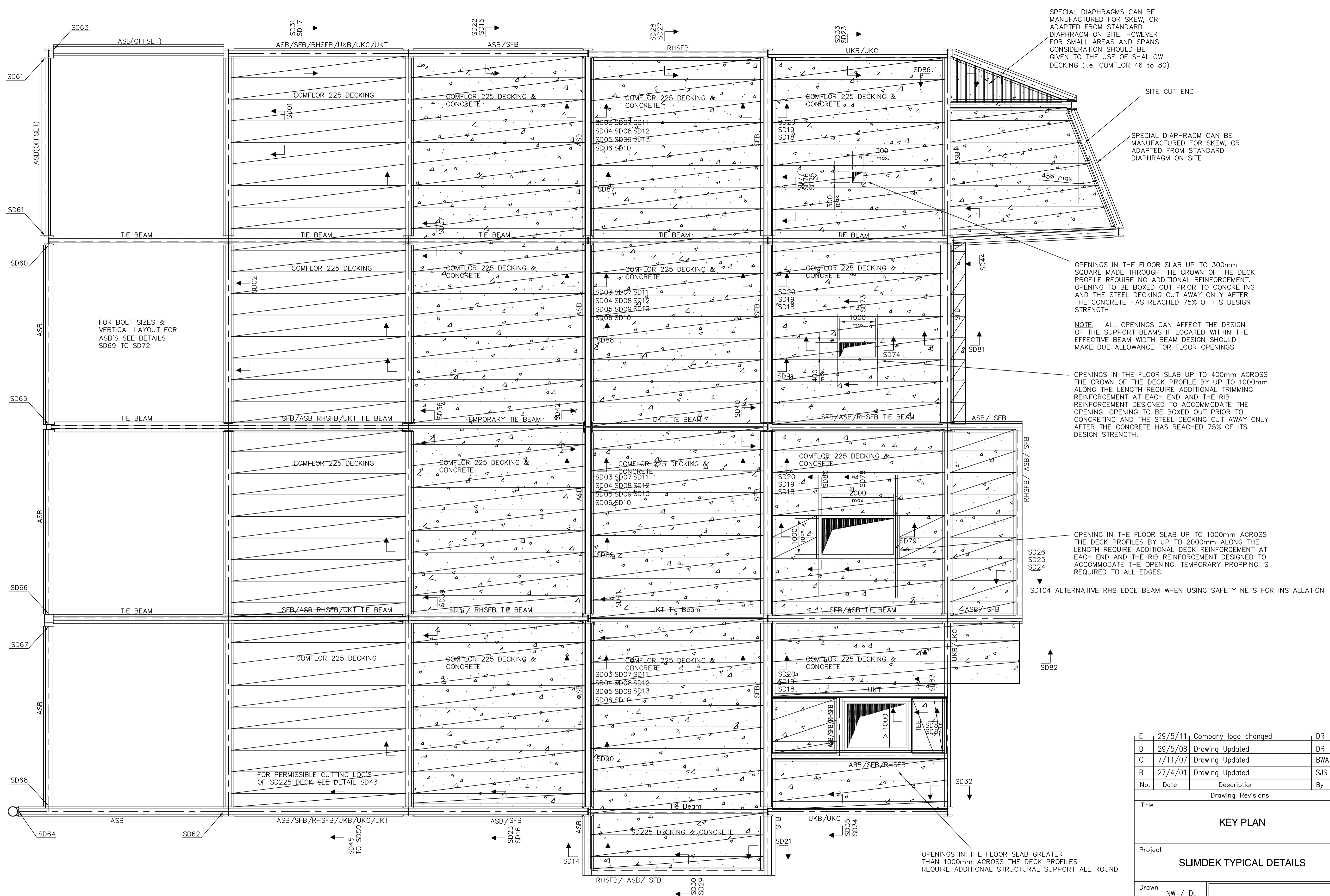
KEY PLAN FOR TYPICAL SLIMDEK DETAILS THIS PLAN IS FOR REFERENCE ONLY
