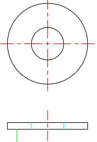
M12 Washer (Type G)
